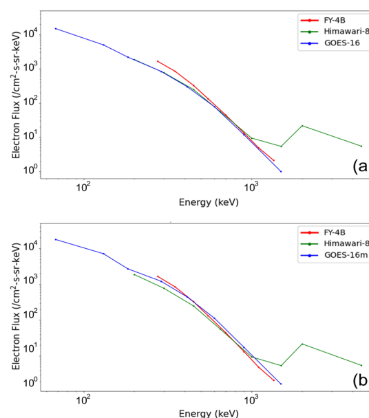
Figure 2. The comparison of flux spectrum between the 3 satellites, 2023/05/18 0:00.
