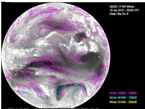
Figure 21. GOES-16 and 17 clear-sky water vapor winds derived from Full Disk 30-minute 6.2um ABI data for 00 UTC on 18 June 2019. These winds are derived from tracking water vapor features using the 6.2um channel. High level (100-400 hPa) winds are shown in violet; mid-level (400-700 hPa) winds are shown in cyan; and low-level winds (below 700 hPa) are shown in yellow.
