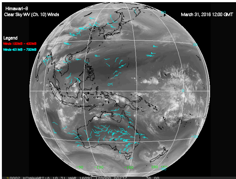
Figure 35. Himawari-8 clear-sky water vapor winds derived from Full Disk 10-minute 7.3um AHI data for 12 UTC on 31 March 2016. These winds are derived from clear-sky water vapor gradients features using the 7.3um channel. Mid-level (400-700 hPa) winds are shown in cyan.
