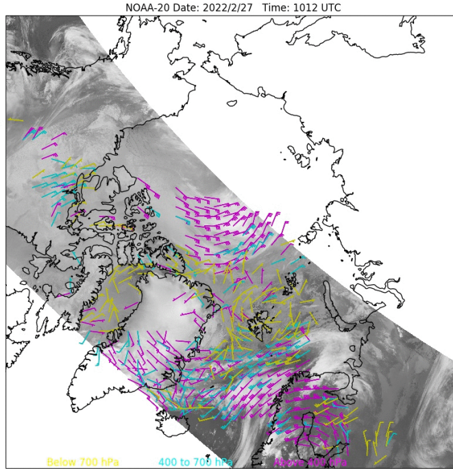
Figure 38. NOAA-20 cloud-drift winds derived in the Arctic from VIIRS Level-1 SDR 10.8um data for 1012 UTC on 27 February 2022. High level (100-400 hPa) winds are shown in violet; mid-level (400-700 hPa) winds are shown in cyan; and low-level winds (below 700 hPa) are shown in yellow.
