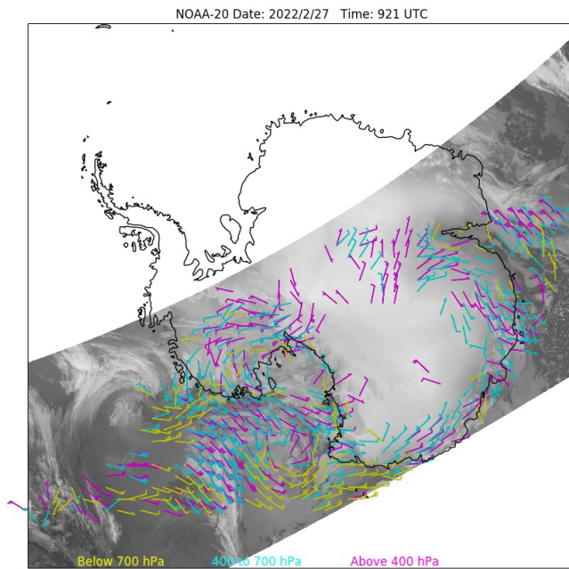
Figure 39. NOAA-20 cloud-drift winds derived in the Antarctic from VIIRS Level-1 SDR 10.8um data for 0921 UTC on 27 February 2022. High level (100-400 hPa) winds are shown in violet; mid-level (400-700 hPa) winds are shown in cyan; and low-level winds (below 700 hPa) are shown in yellow.
