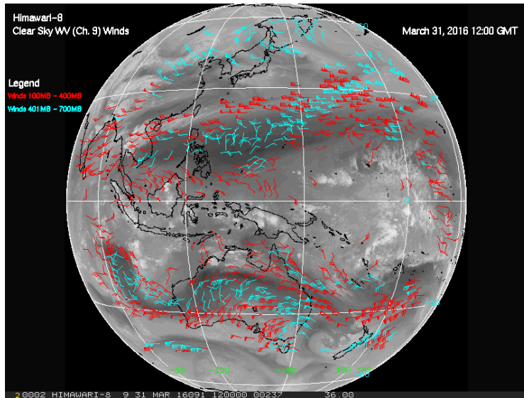
Figure 34. Himawari-8 clear-sky water vapor winds derived from Full Disk 10-minute 6.9um AHI data for 12 UTC on 31 March 2016. These winds are derived from clear-sky water vapor gradients features using the 6.9um channel. High level (100-400 hPa) winds are shown in red and mid-level (400-700 hPa) winds are shown in cyan.
