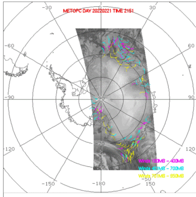
Figure 41. Metop-C cloud-drift winds derived in the Antarctic from AVHRR-3 L1b 10.8um data for 2151 UTC on 21 February 2022. High level (100-400 hPa) winds are shown in violet; mid-level (400-700 hPa) winds are shown in cyan; and low-level winds (below 700 hPa) are shown in yellow.
