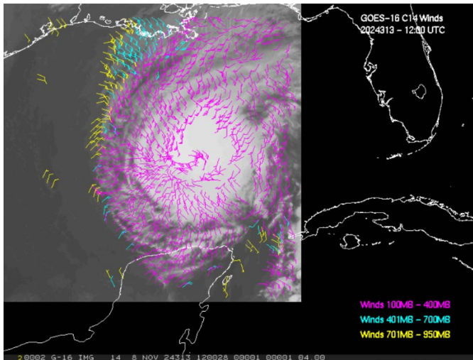
Figure 30. GOES-16 high resolution (spatiotemporal) cloud-drift winds derived from MESO sector 1-minute ABI 11.2um data for 12 UTC on 08 November 2024. High level (100-400 hPa) winds are shown in violet; mid-level (400-700 hPa) winds are shown in cyan; and low-level winds (below 700 hPa) are shown in yellow. NOTE: the plotted high resolution vectors shown in this image have been thinned for visual clarity.
