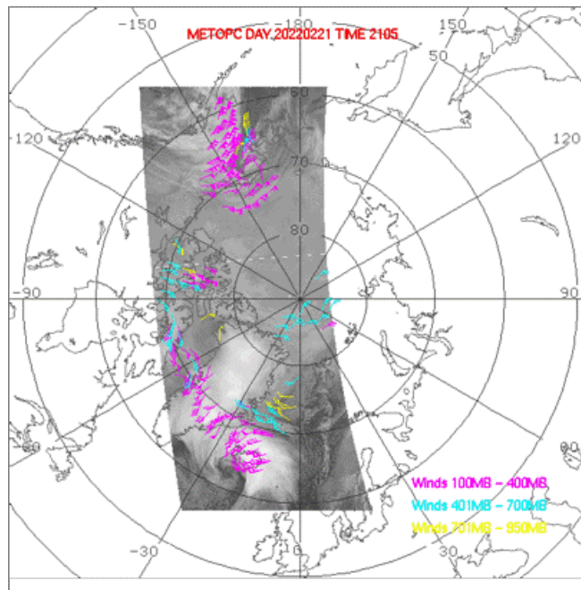
Figure 40. Metop-C cloud-drift winds derived in the Arctic from AVHRR-3 L1b 10.8um data for 2105 UTC on 21 February 2022. High level (100-400 hPa) winds are shown in violet; mid-level (400-700 hPa) winds are shown in cyan; and low-level winds (below 700 hPa) are shown in yellow.
