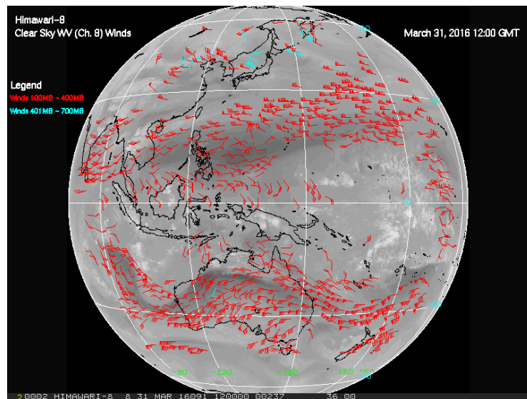
Figure 33. Himawari-8 clear-sky water vapor winds derived from Full Disk 10-minute 6.2um AHI data for 12 UTC on 31 March 2016. These winds are derived from clear-sky water vapor gradients features using the 6.2um channel. High level (100-400 hPa) winds are shown in red and mid-level (400-700 hPa) winds are shown in cyan.
