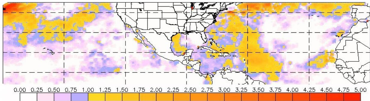
Fig. 10. HotSpot Product of Sea-Surface Temperature
