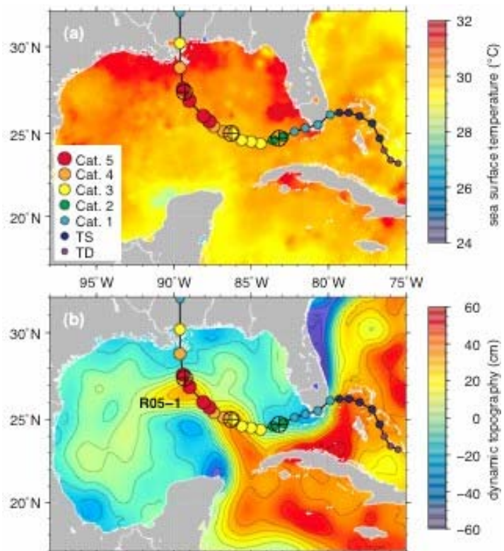
Fig. 19. Hurricane Katrina intensified from Category 2 to 5 when it crossed regions of high oceanic heat content, which are regions of high topography detectable by satellite altimetry (lower map). Coincident sea surface temperature data (top map) does not clearly suggest hurricane intensification.
