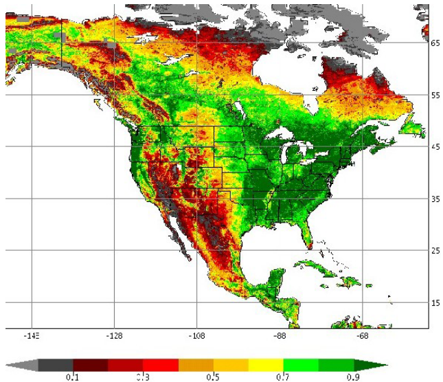
Fig. 17. A Green Vegetation Fraction product in June
