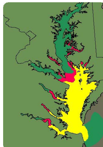
Fig. 14. Relative abundance of an algal species harmful to fish, in Chesapeake Bay, April 2005.
