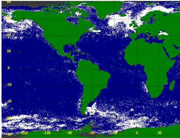
Fig. 12. Abundance (in white) of the phytoplankton species Emiliana huxlevi in SeaWiFS satellite
