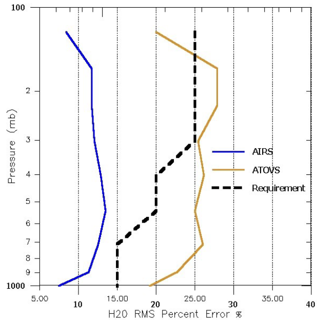
Fig. 30. Error comparison of two instruments (AIRS and ATOVS) at various heights (pressures) in the atmosphere.
