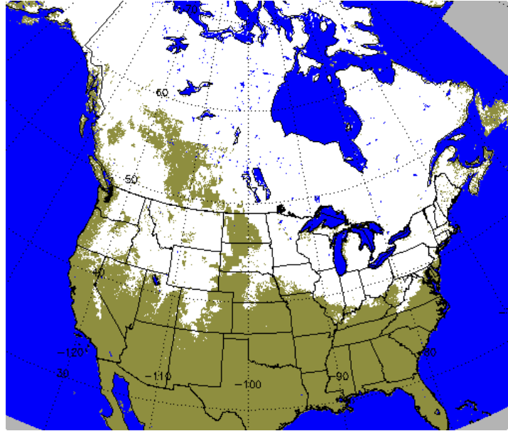
Fig. 24. Daily Snow Cover Map by NESDIS for Dec. 14, 2005
