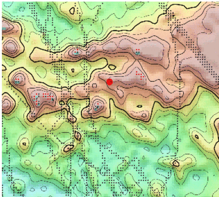
Fig. 27. Depth contours of central Pacific Ocean based on both conventional soundings (black dots) and satellite altimetry. Submarine crashed near the large red dot. This chart spans 350 km from left to right.
