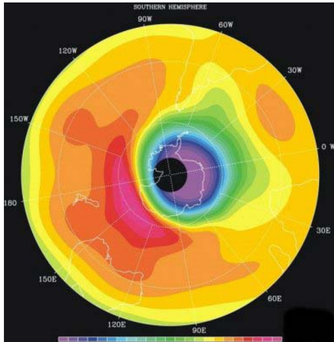
Fig. 21. Ozone concentration in southern hemisphere stratosphere, SBUV-2 sensor, NOAA satellite, Oct 2001.
