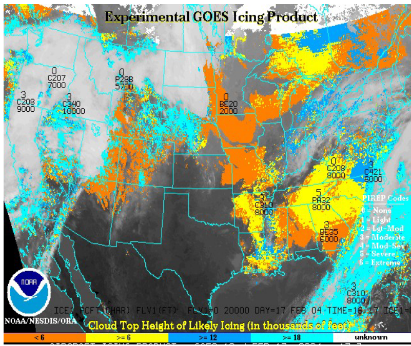
Fig. 25. Experimental GOES satellite product for Aviation Icing
