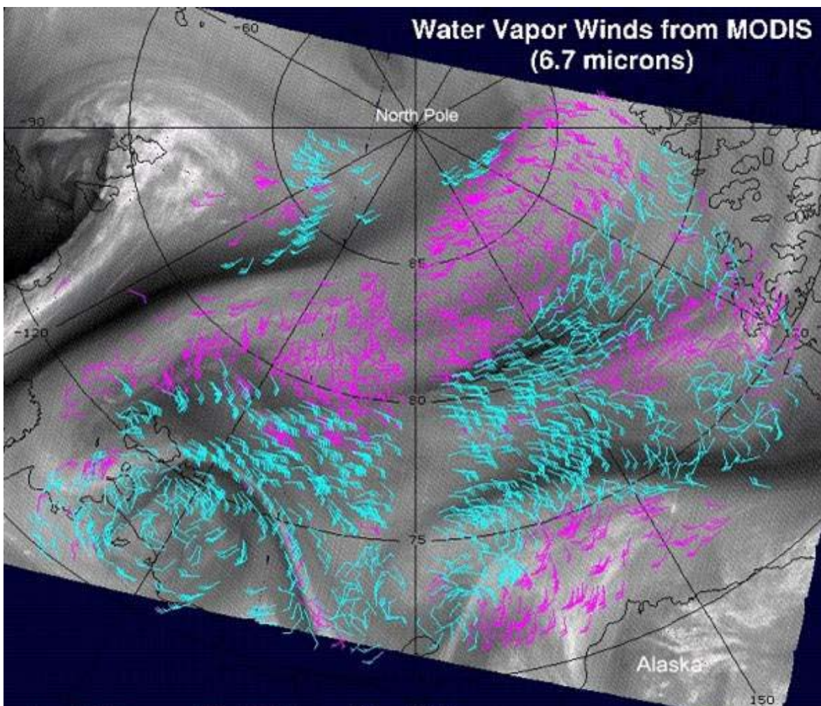
Fig. 18. Winds derived from motion of features on MODIS images
