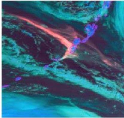
Fig. 26. Volcanic ash (in red) on a satellite product using MODIS data.
