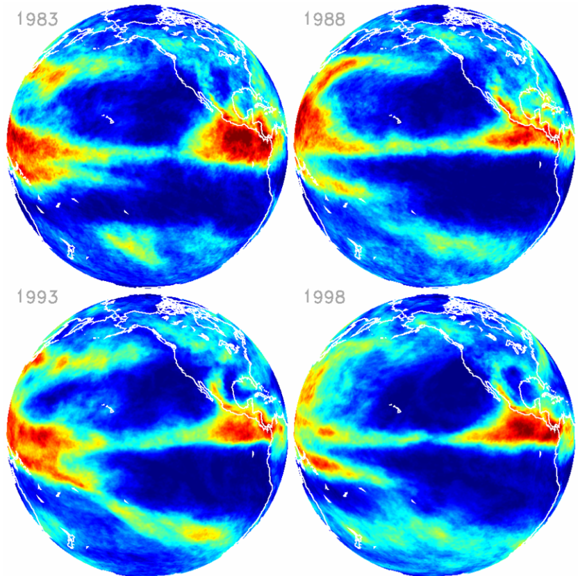
Fig. 15. Example of a new climate data set from reprocessing polar orbiting images. The globes show the year-to-year variability in high clouds from data in July for four different years, 1983, 1988, 1993 and 1998. Areas with large amounts of high cloud are red, while areas with less high cloud are blue.
