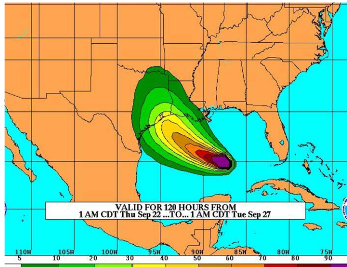
Fig. 20. Probability (%) of winds exceeding hurricane force in a five-day period, in September 2005 for Hurricane Rita
