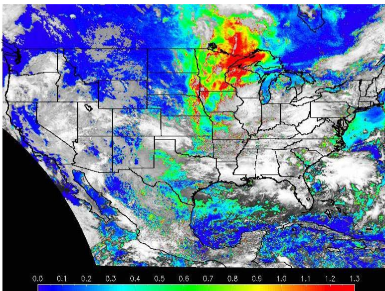
Fig. 23. Aerosol Monitoring for Air Quality and Forecasting
