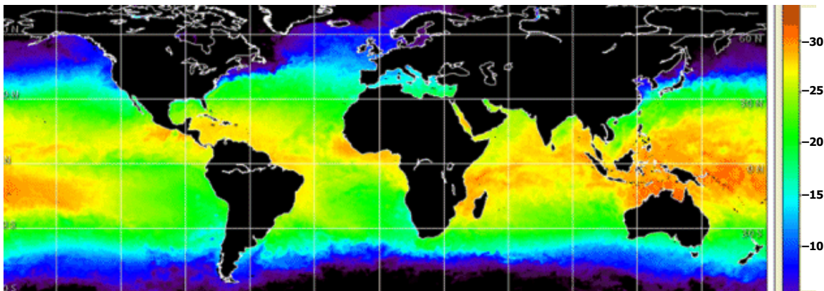
Fig. 16. New STAR Sea-Surface Temperature daily product blending polar (POES) and geostationary (GOES) satellite temperature observations for the entire globe.
