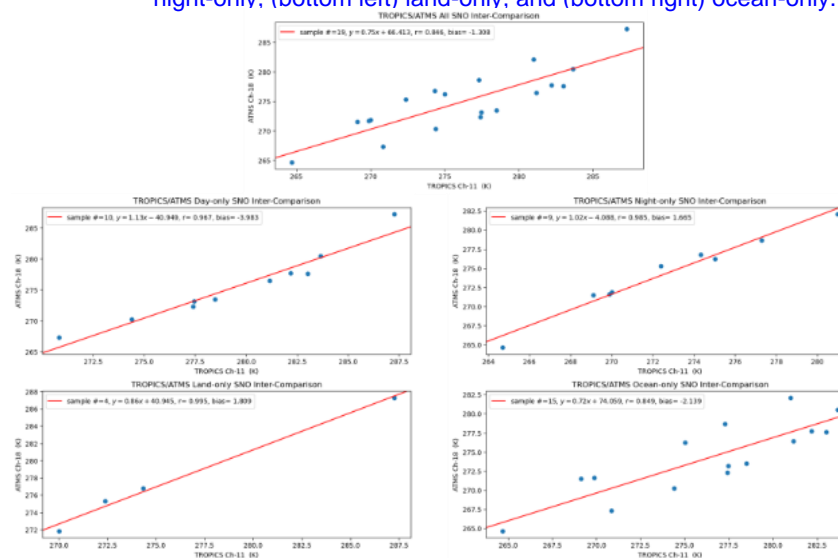
Figure 1. ATMS Ch 18 versus TROPICS Ch 11 brightness temperatures for Simultaneous Nadir Overpasses (SNOs) occurring August 8-9, 2021 for the (top) globe, (middle left) day-only, (middle right) night-only, (bottom left) land-only, and (bottom right) ocean-only.
