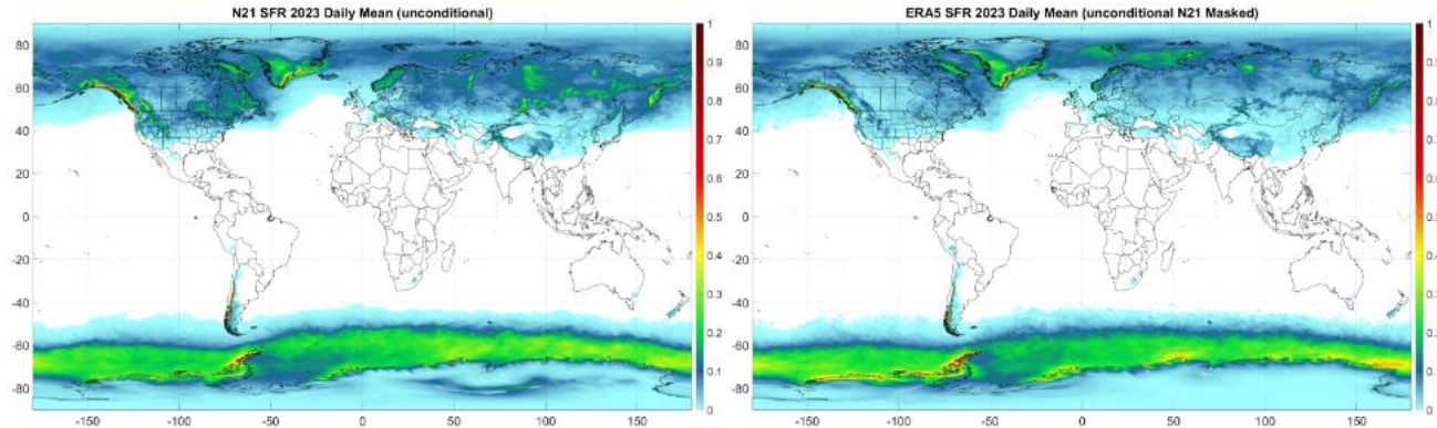
Comparison of snowfall rate daily mean between NOAA-21 (left) and ECMWF reanalysis ERA5 (right). The two products agree well with each other in most regions of the globe.
