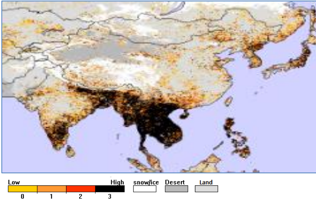
Figure. Thermal Stress Map of VIIRS Vegetation Thermal Condition Index (TCI) of Eastern Asia for the week 18 of 2024. The black areas are suffering exceptional thermal stress.
